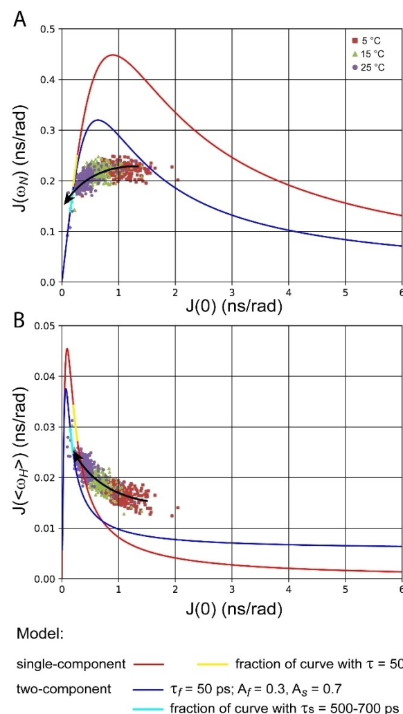
Figure 4. Spectral density analysis of ^{15}\text{N} NMR relaxation rates of tau protein, in dependence of temperature. The J(\omega_N) vs. J(0) (A) and J(<\omega_H>) vs. J(0) (B) relations at 5 (red squares), 15 (green triangles) and 25 °C (purple circles) show a clear deviation from the theoretical relation expected for a single or two-Lorentzian motion (solid red and blue curves). However, the general trend (black arrows) suggests that with a temperature rising above 25 °C, the J(\omega_N) or J(<\omega_H>) vs. J(0) relations might be pushed towards the theoretical single or two-Lorentzian curves (red or blue lines, correspondingly). See text for further details.
